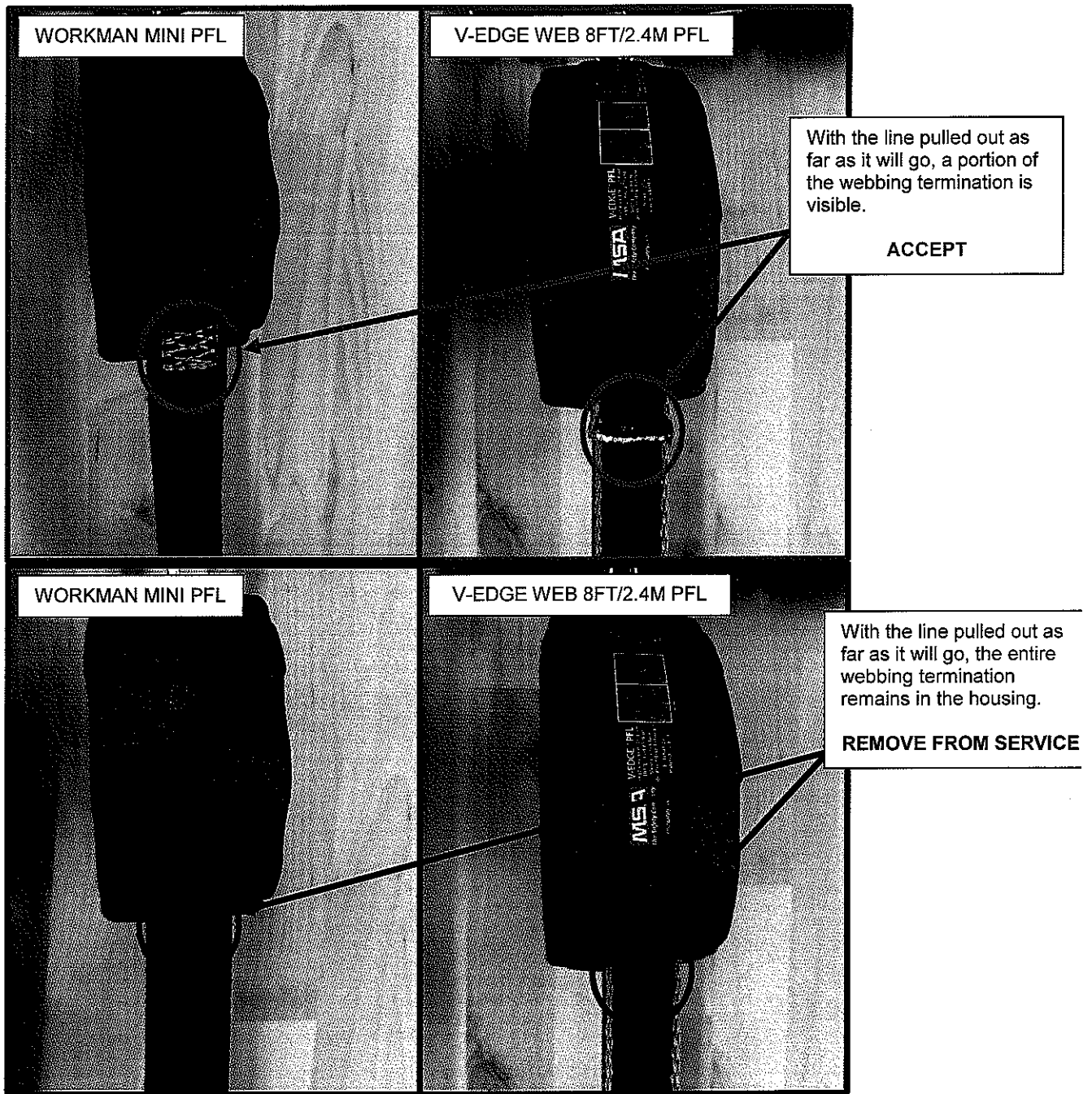
Figure 2 – Webbing Termination
